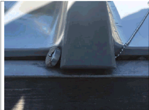
Toggle entrapment at top of slide
